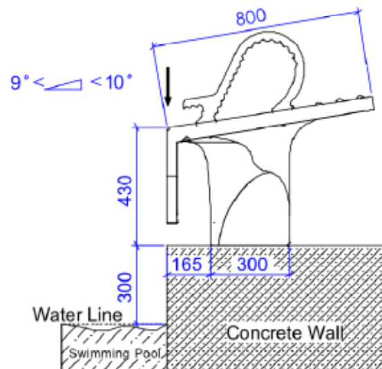
Technical Drawing of SuperBlock
