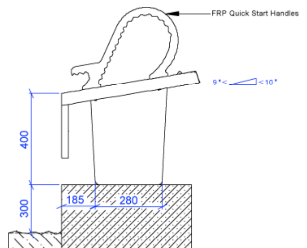
Technical Drawing of Anti Block
