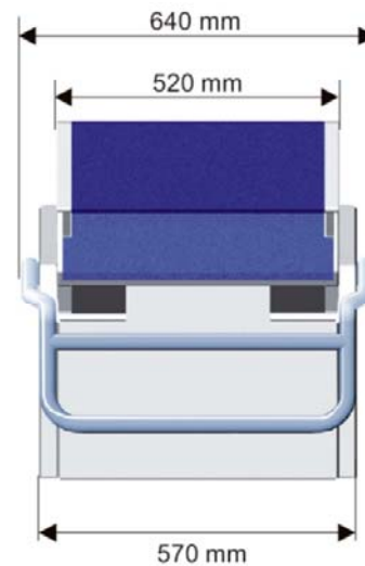
OMEGA OSB11 START BLOCK
